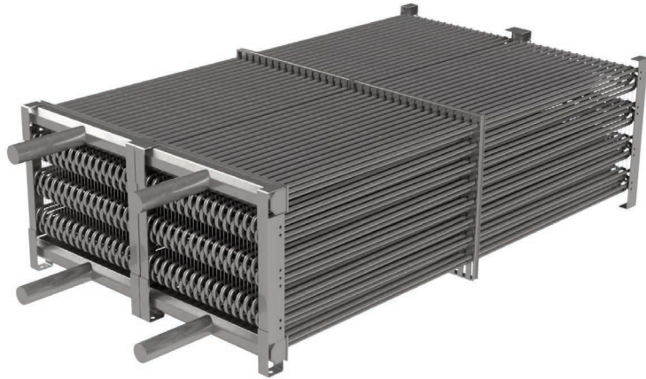
ASME B31.5 STAINLESS STEEL CONDENSER COIL
